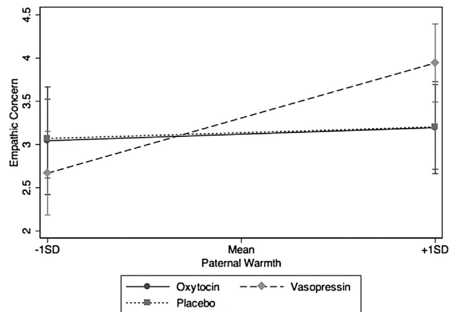
Figure 1 There was a significant interaction of drug condition (AVP, OT, placebo) \times paternal warmth on empathic concern following the distressing video. At +1 SD above the mean of paternal warmth, individuals on AVP reported significantly higher levels of empathic concern compared to those on placebo or OT. Error bars represent 95% CIs.
